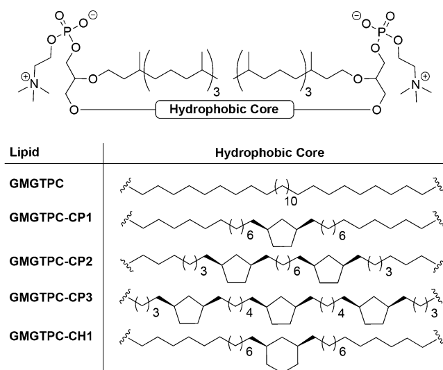
Scheme 1. Structures of synthesized tetraether lipids.
